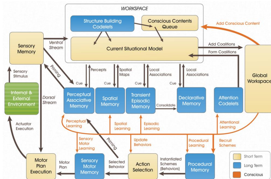
Fig. 8.2 The LIDA Cognitive Cycle
